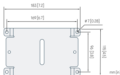
Indigo500 retrofit mounting plate dimensions
