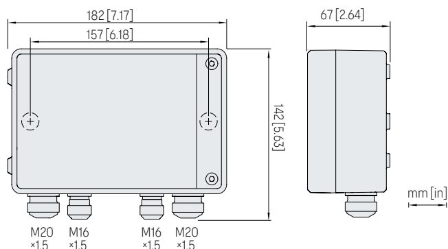
Indigo520 Supervisor dimensions and lead-through sizes
